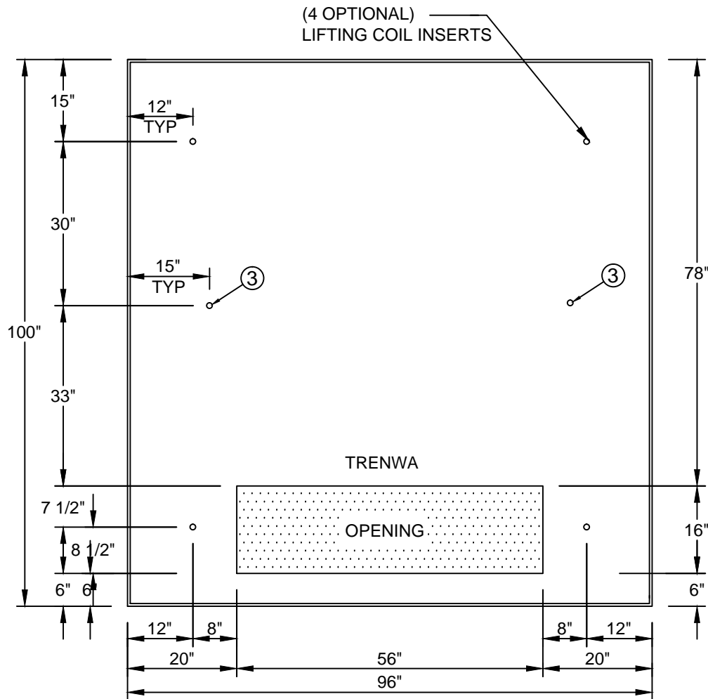
PLAN VIEW
