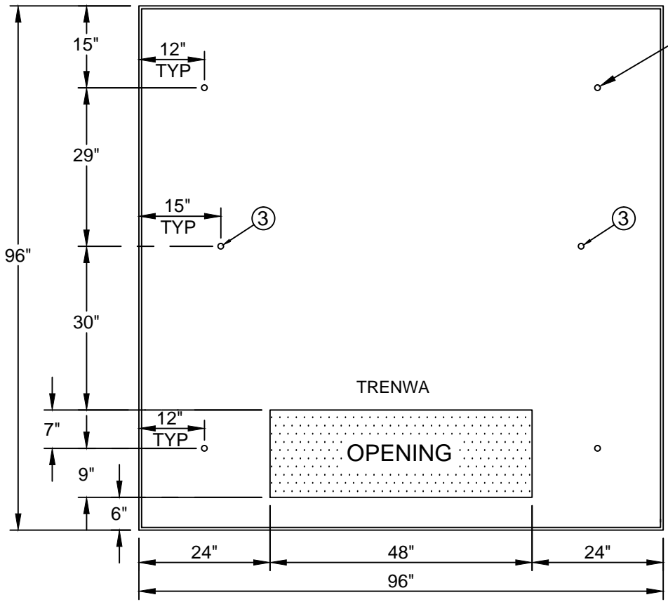
PLAN VIEW
