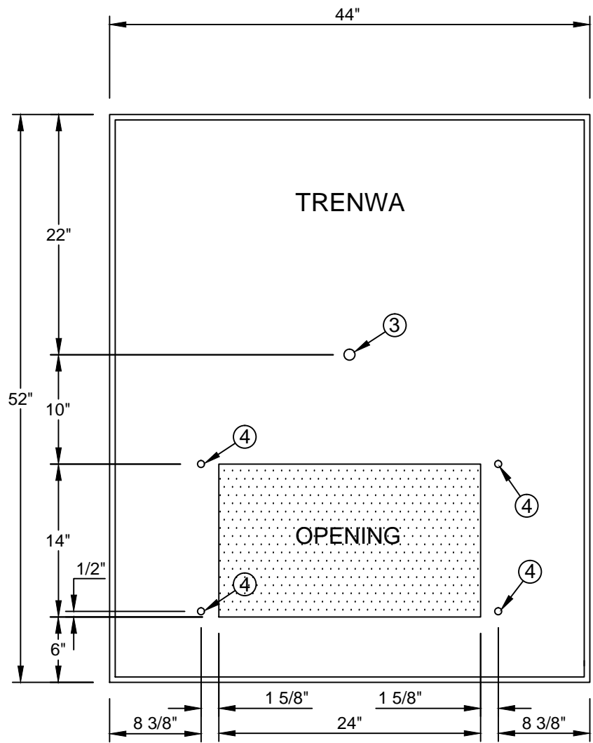
PLAN VIEW
