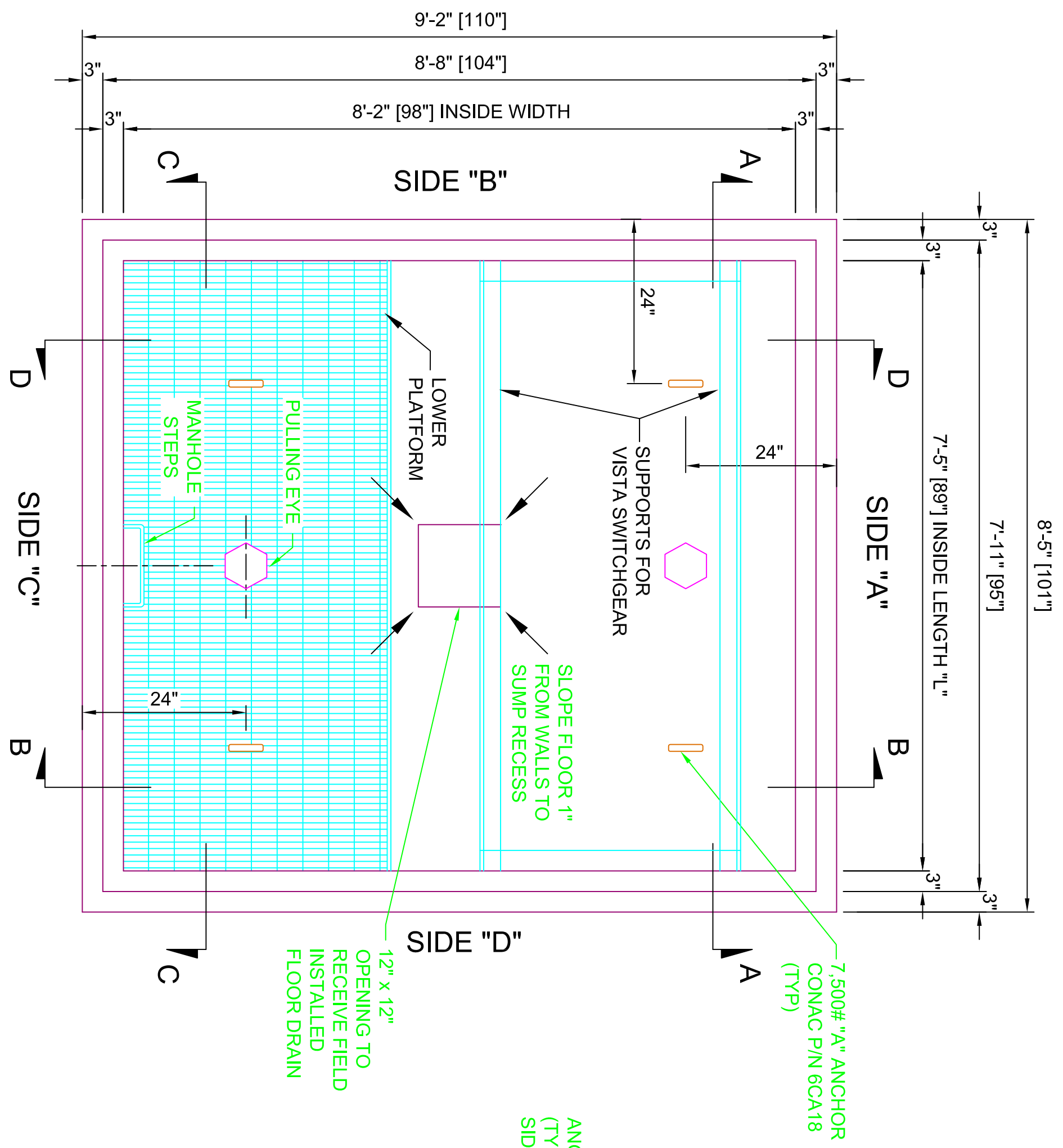
PLAN VIEW (ANGLE SUPPORTS OMITTED FOR CLARITY)
