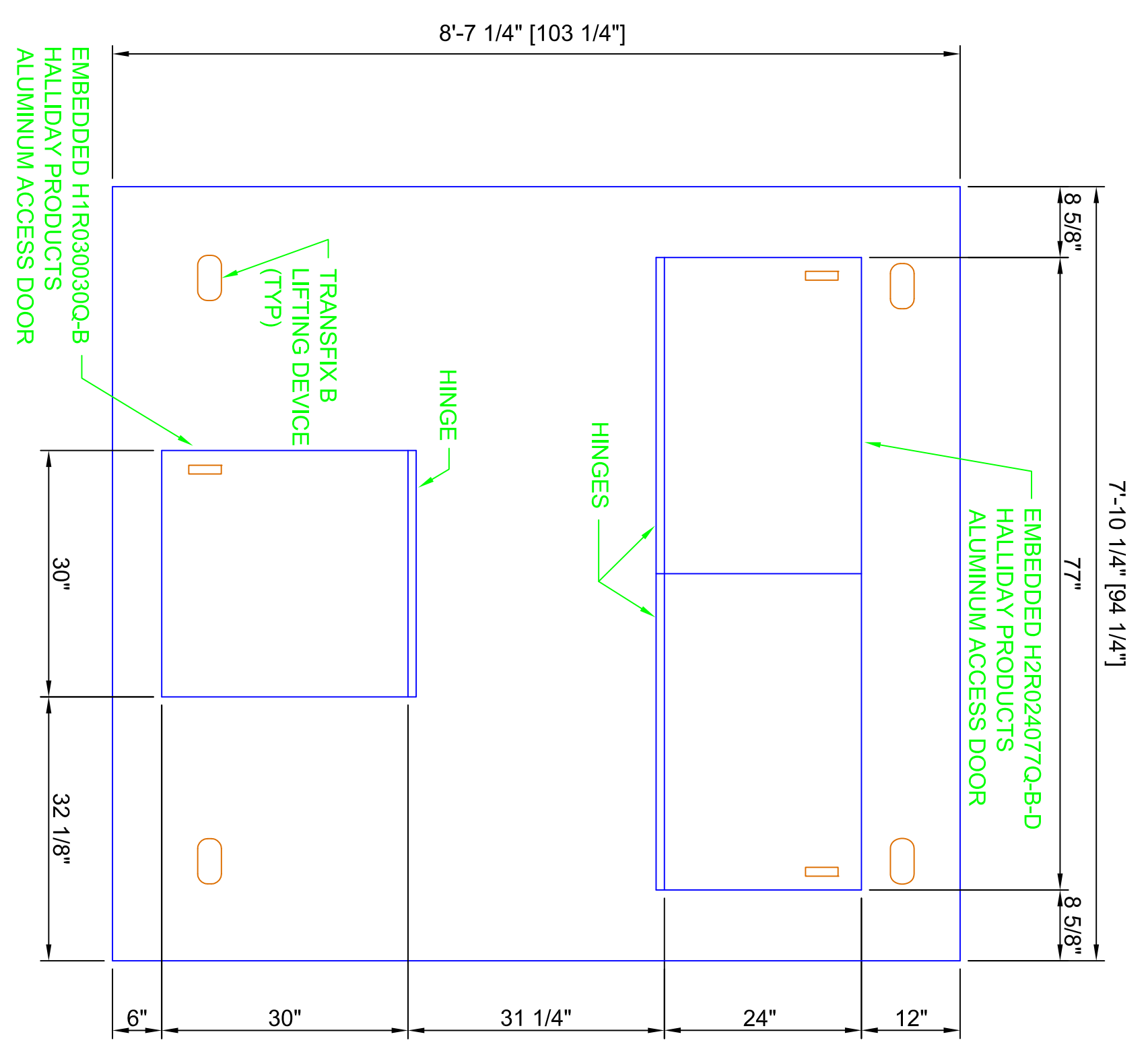
CONCRETE - LID 300 PSF LIVE LOAD (NOT DESIGNED FOR VEHICULAR TRAFFIC)
