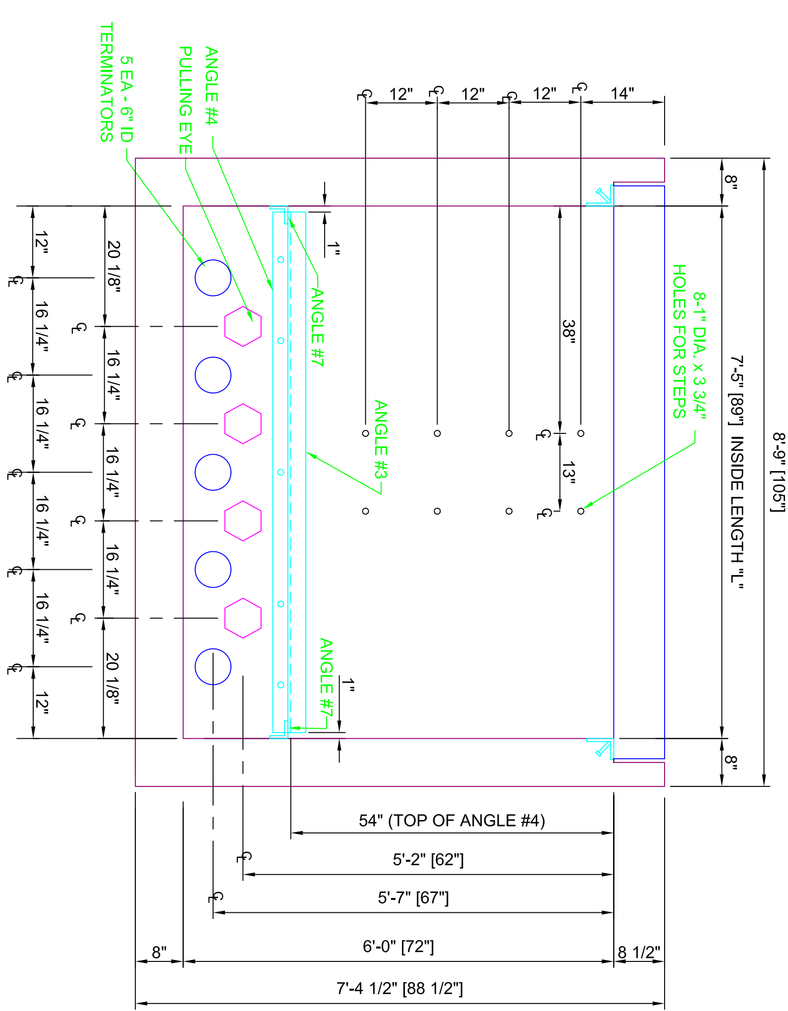
SECTION VIEW C-C (STANDING INSIDE BOX)
