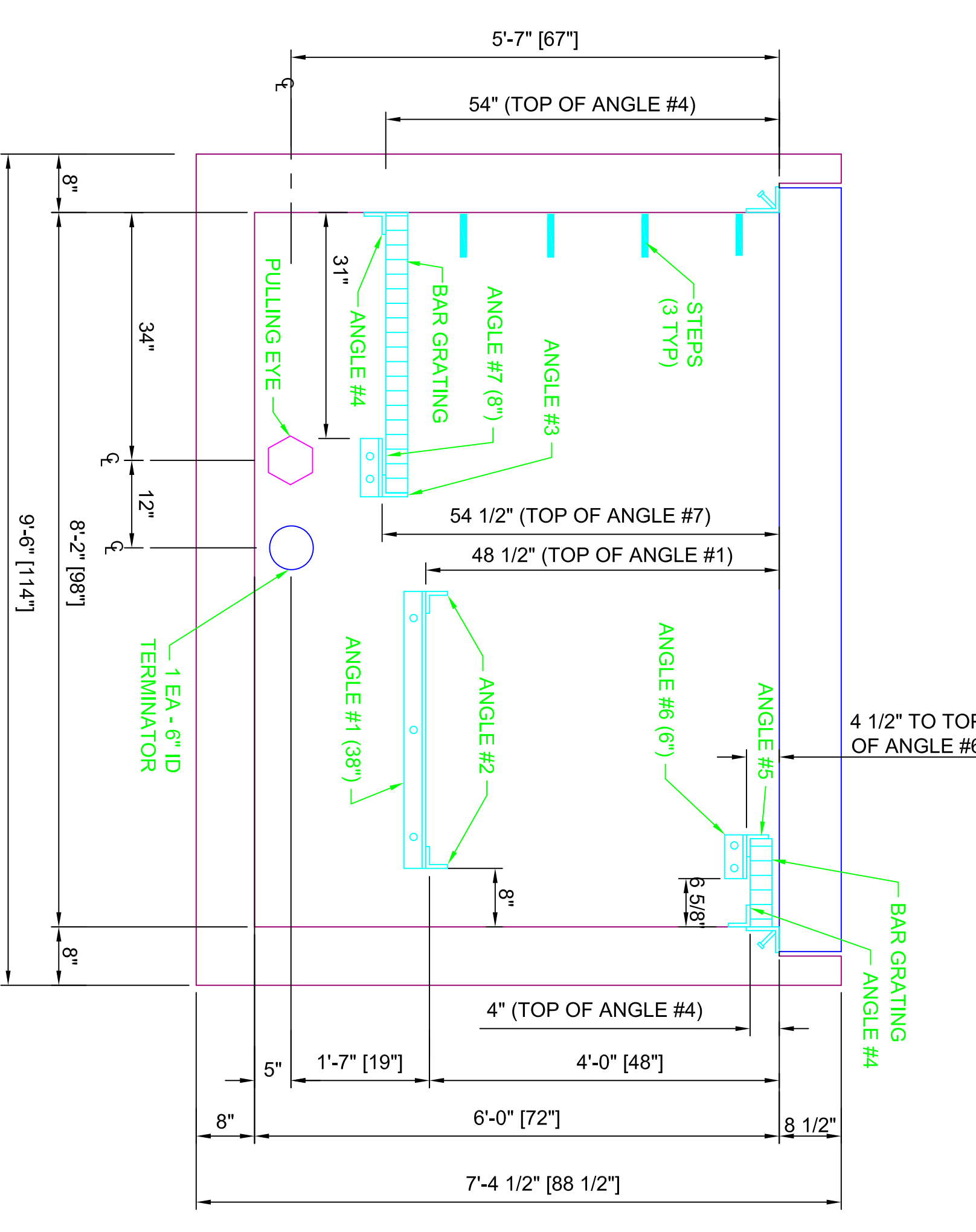
SECTION VIEW B-B (STANDING INSIDE BOX)
