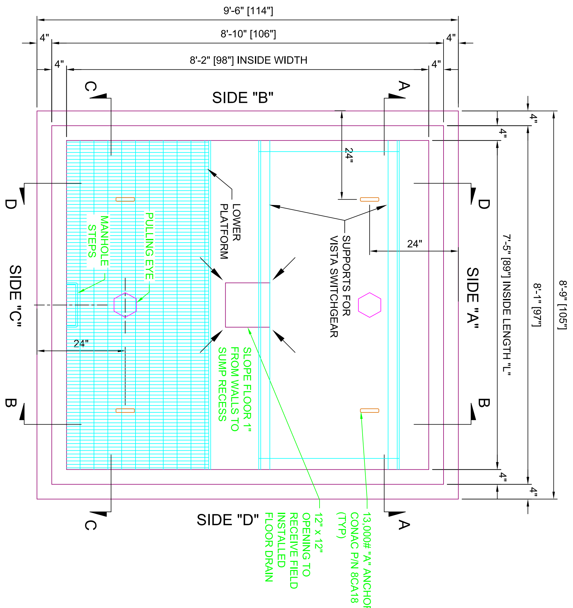
PLAN VIEW (ANGLE SUPPORTS OMITTED FOR CLARITY)
