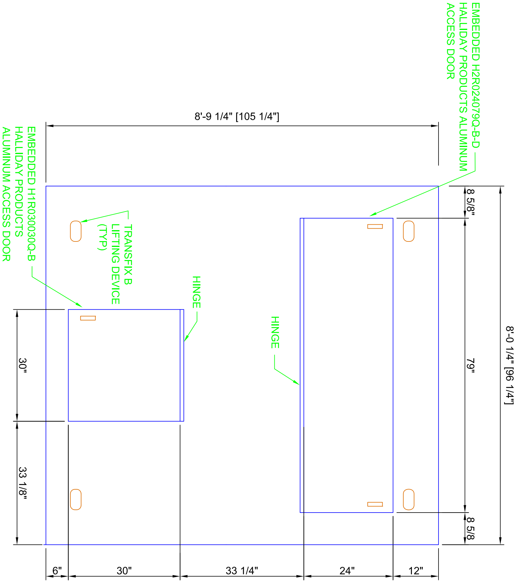
CONCRETE - LID HS20 HIGHWAY LOAD
