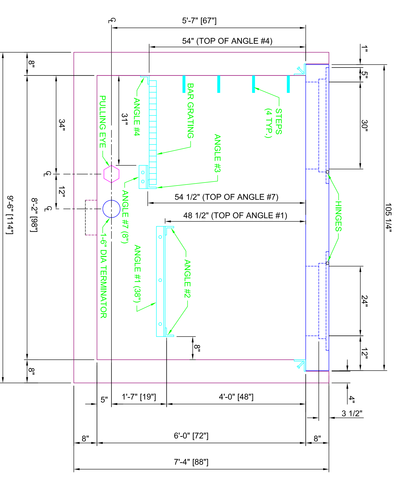
SECTION VIEW B-B (STANDING INSIDE BOX)
