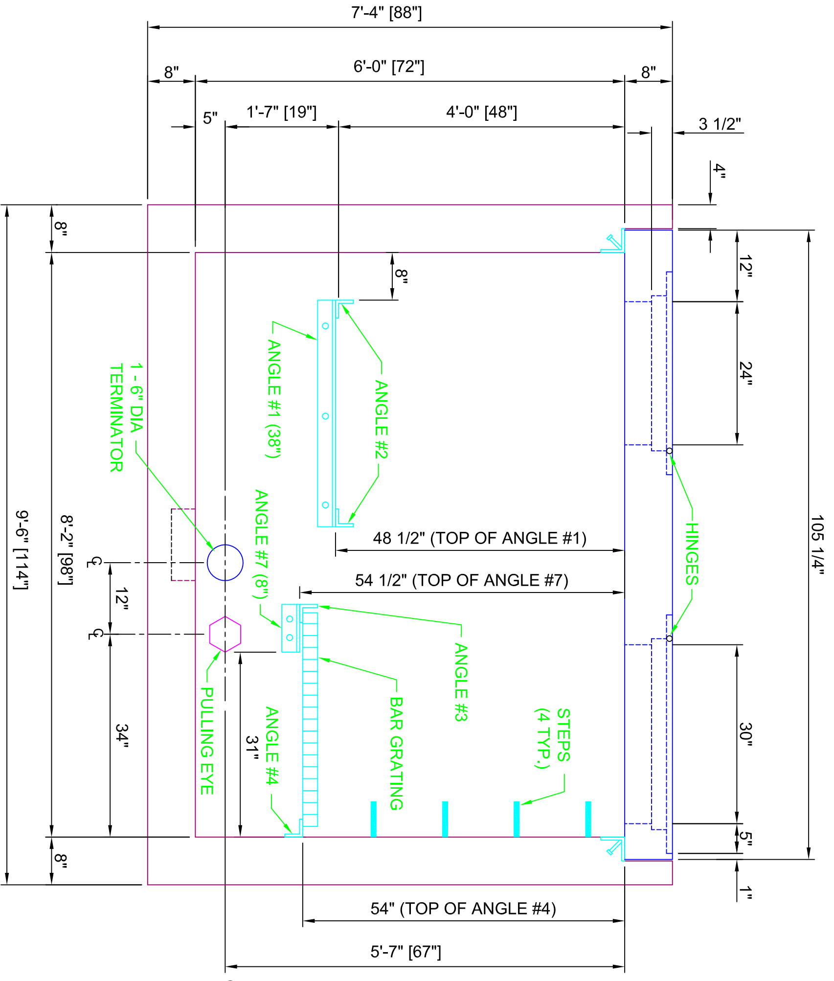
SECTION VIEW D-D (STANDING INSIDE BOX)
