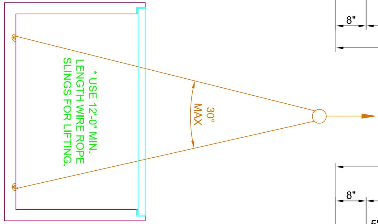
LIFTING DETAIL
