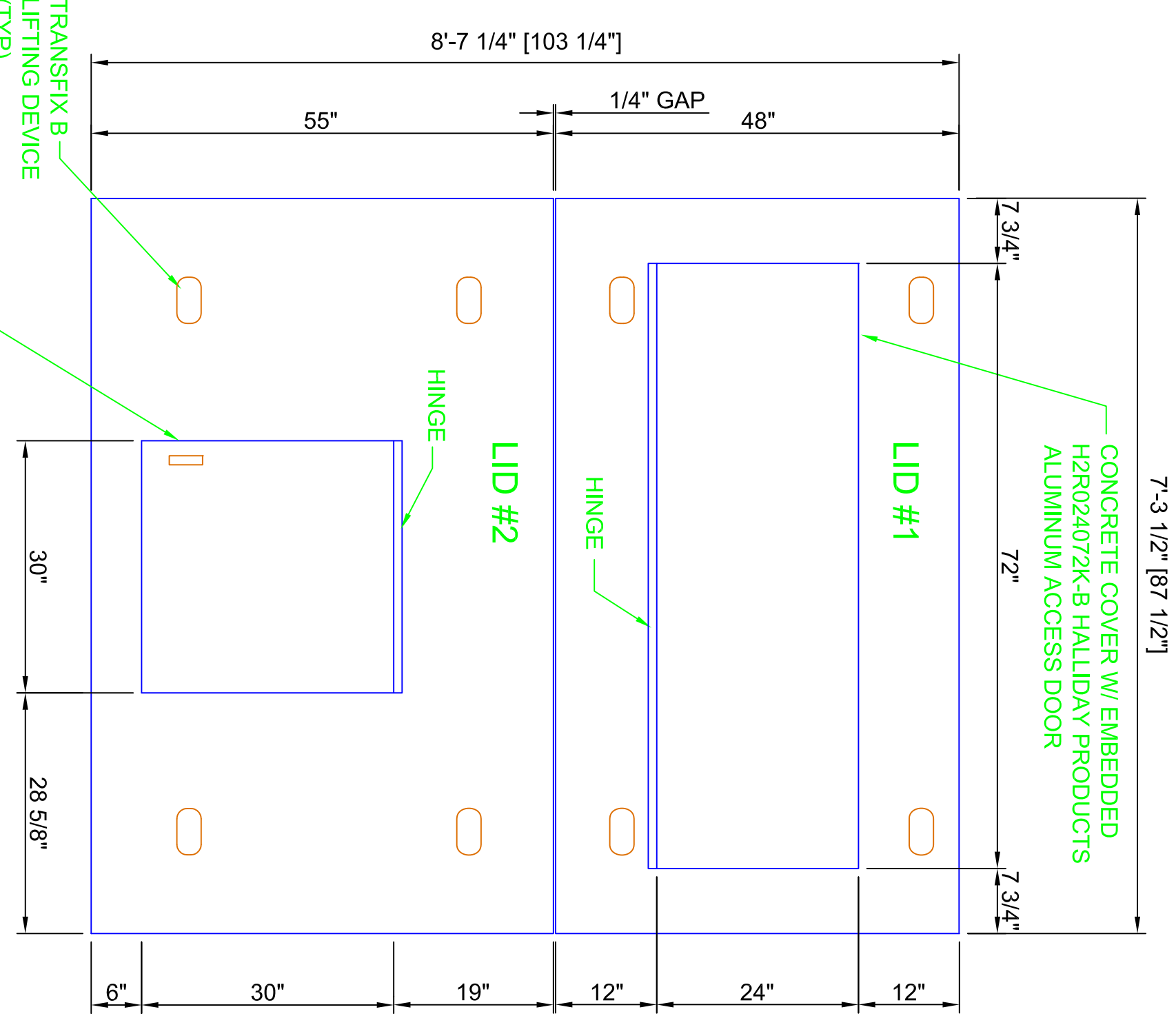
PLAN VIEW (ANGLE SUPPORTS OMITTED FOR CLARITY)
