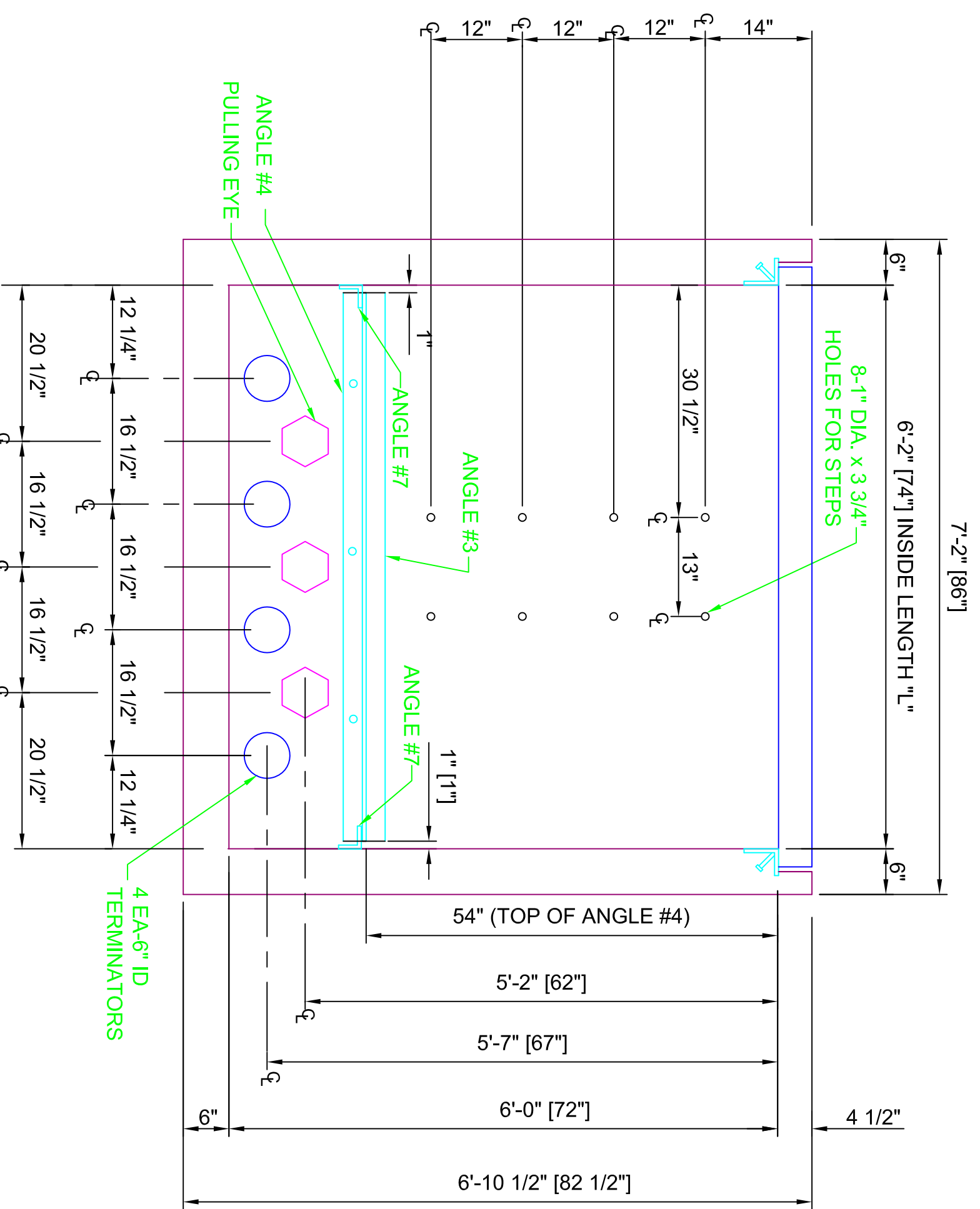
SECTION VIEW C-C (STANDING INSIDE BOX)
