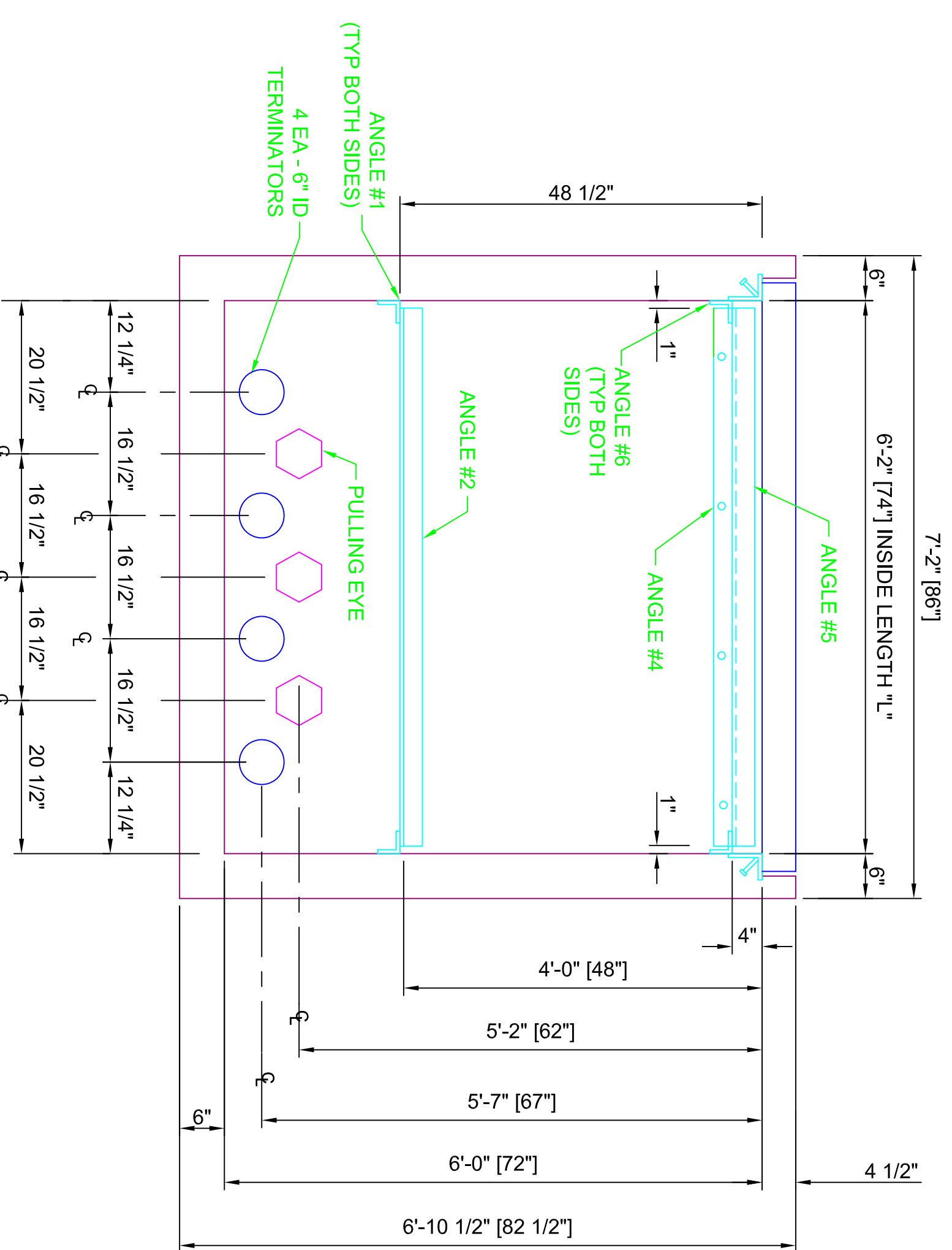
SECTION VIEW A-A (SWITCH GEAR END STANDING INSIDE BOX)
