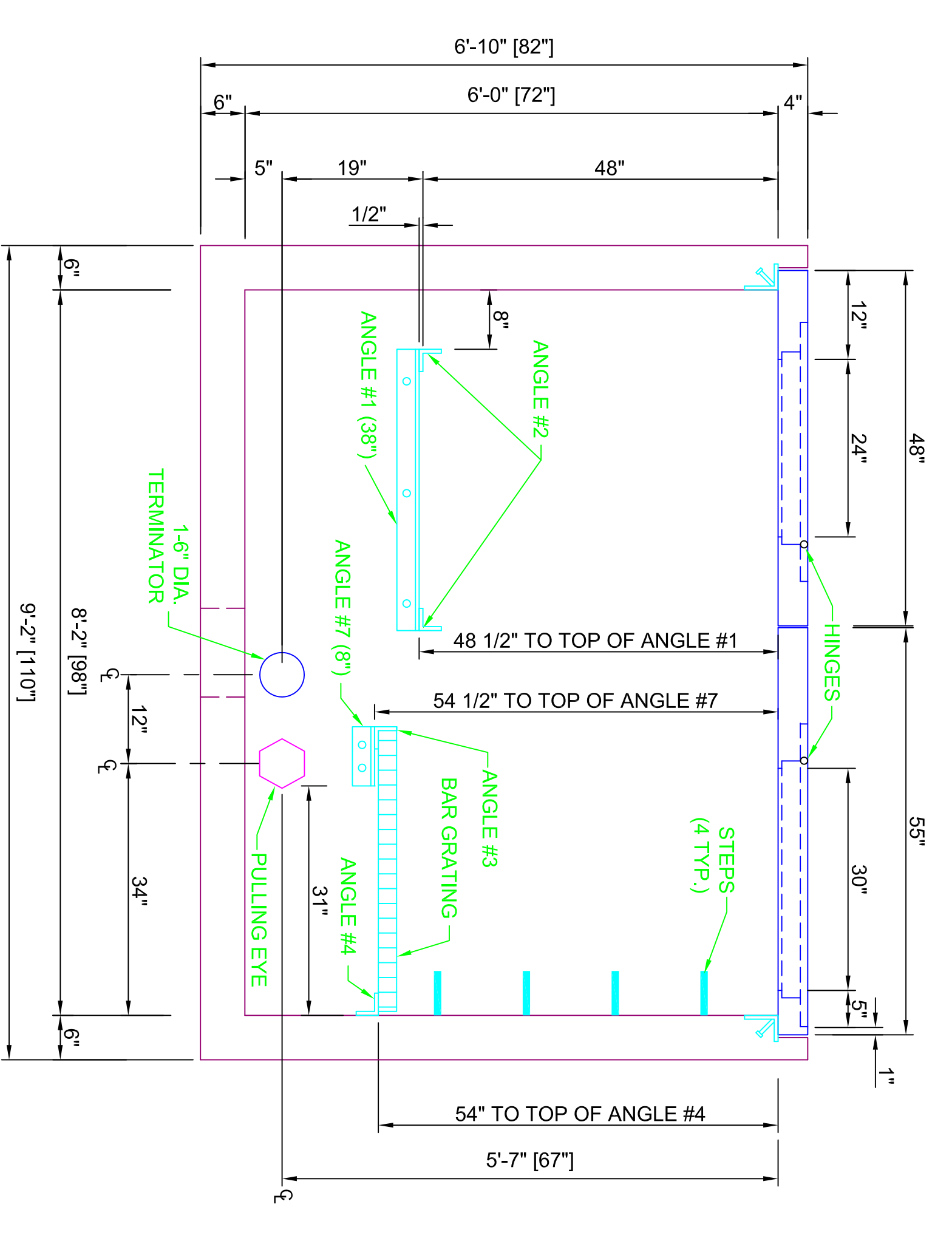
SECTION VIEW D-D (STANDING INSIDE BOX)
