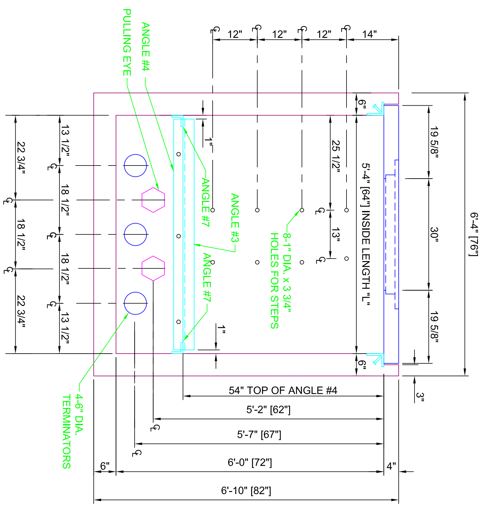
SECTION VIEW C-C (STANDING INSIDE BOX)
