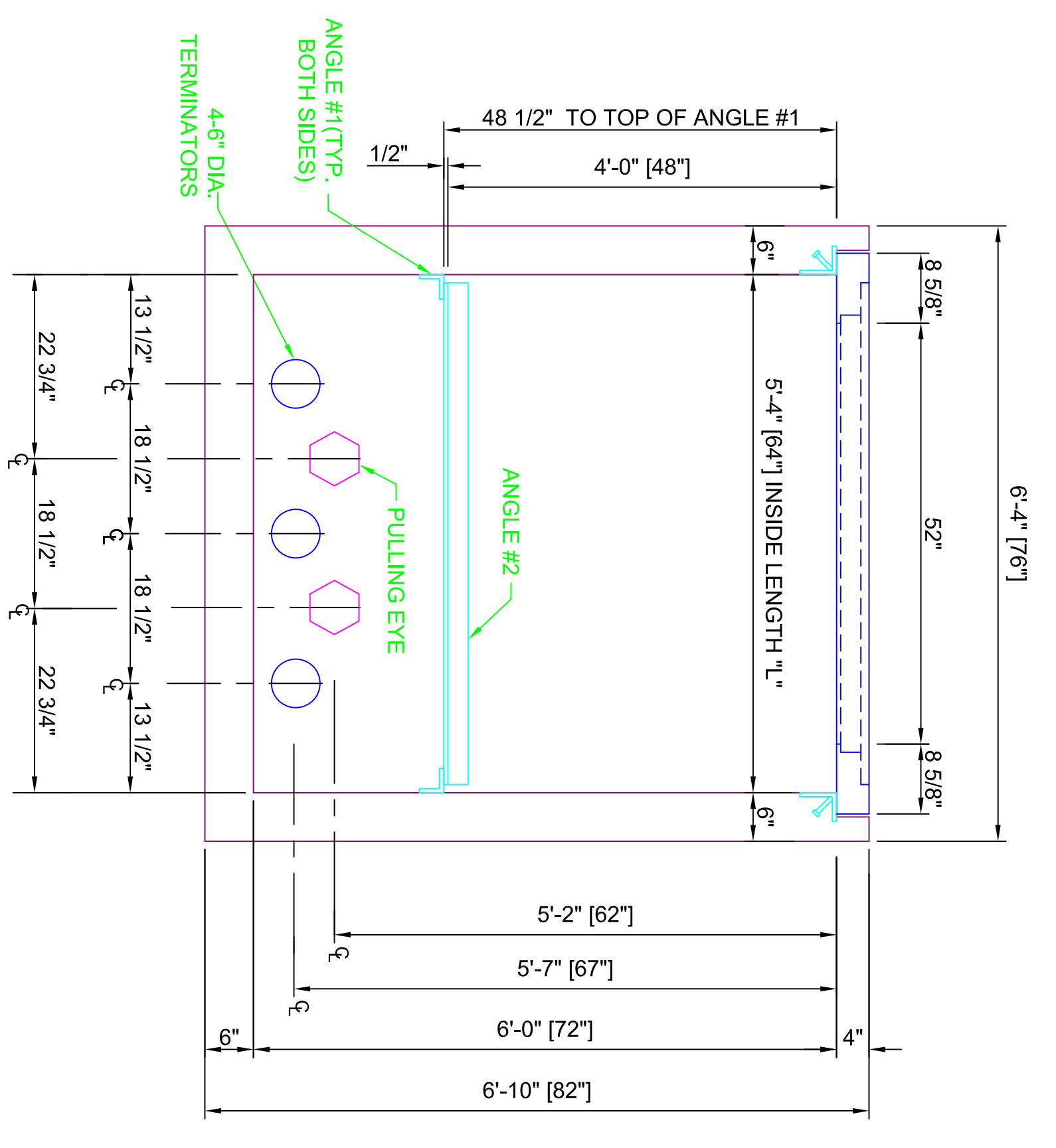
SECTION VIEW A-A (SWITCH GEAR END (STANDING INSIDE BOX))
