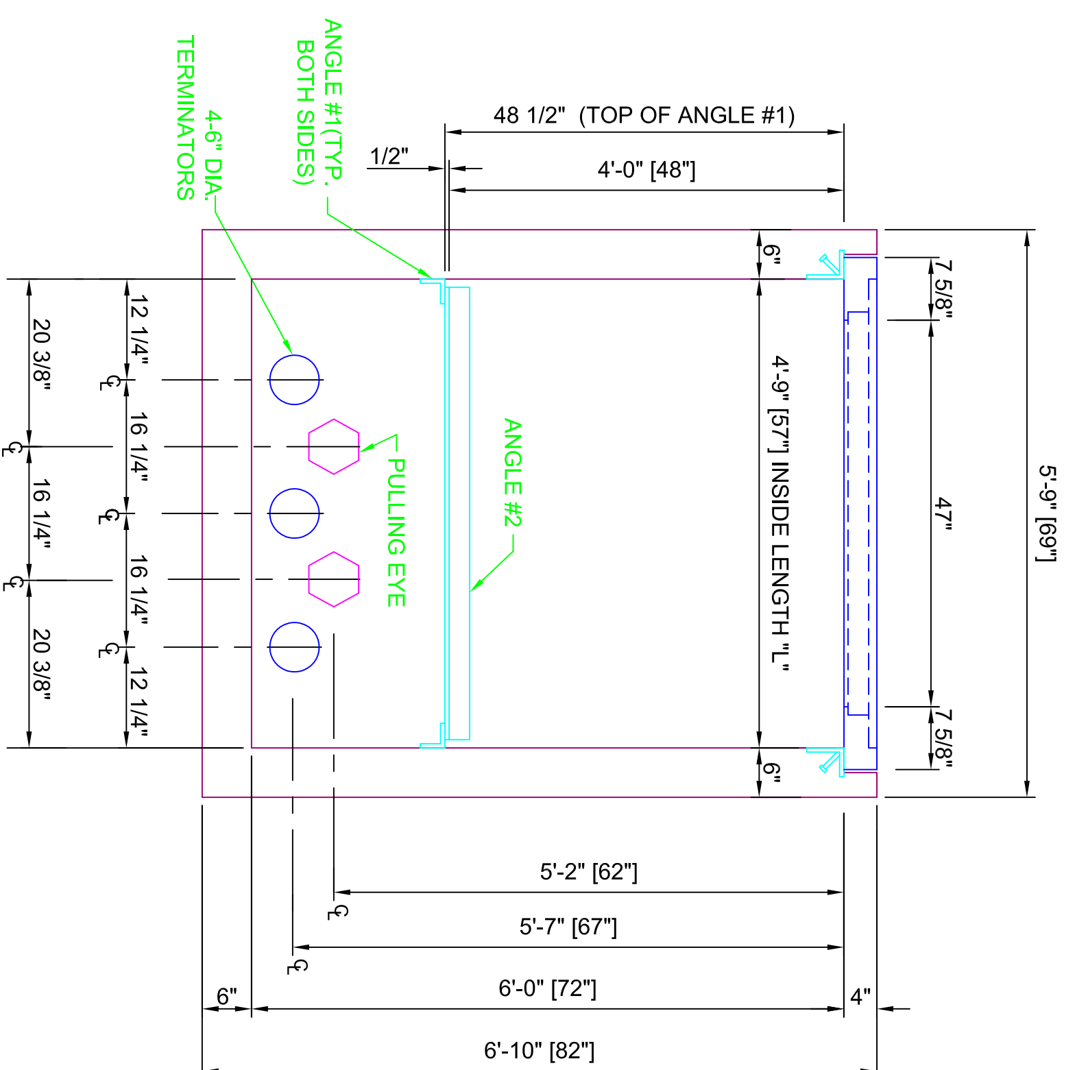
SECTION VIEW A-A (STANDING INSIDE BOX)
