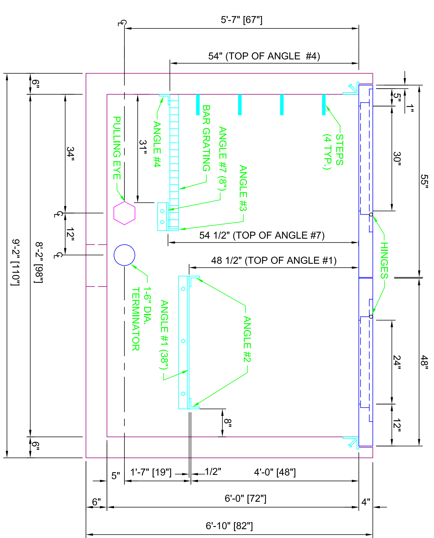
SECTION VIEW B-B (STANDING INSIDE BOX)
