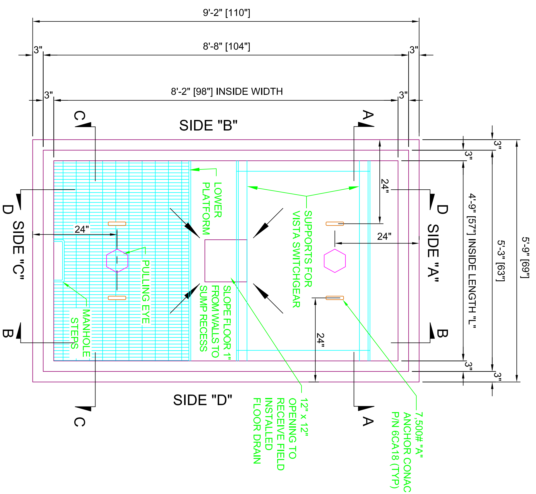
PLAN VIEW (ANGLE SUPPORTS OMITTED FOR CLARITY)
