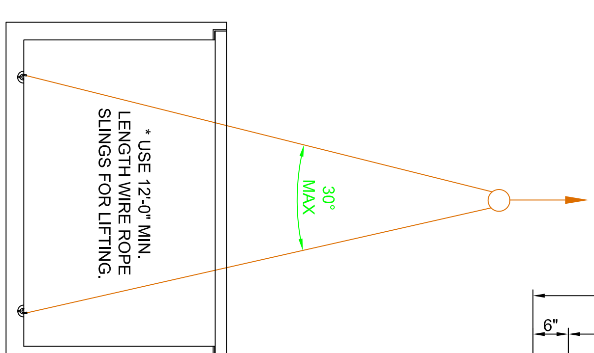
LIFTING DETAIL
