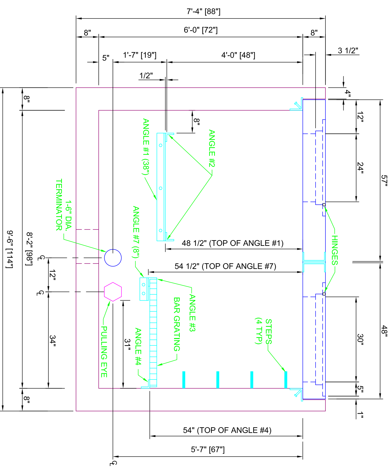
SECTION VIEW D-D (STANDING INSIDE BOX)
