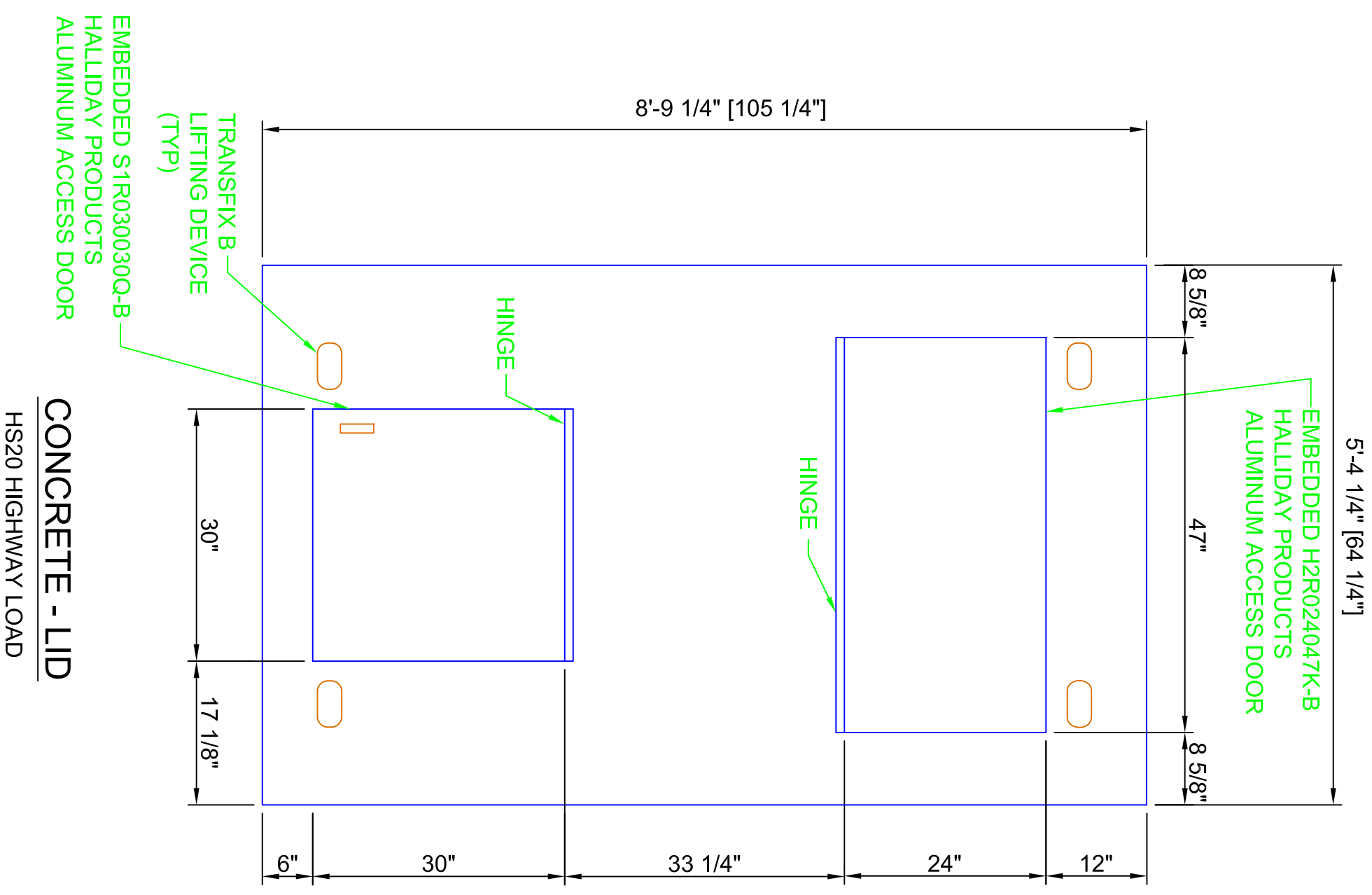
PLAN VIEW (ANGLE SUPPORTS OMITTED FOR CLARITY)
