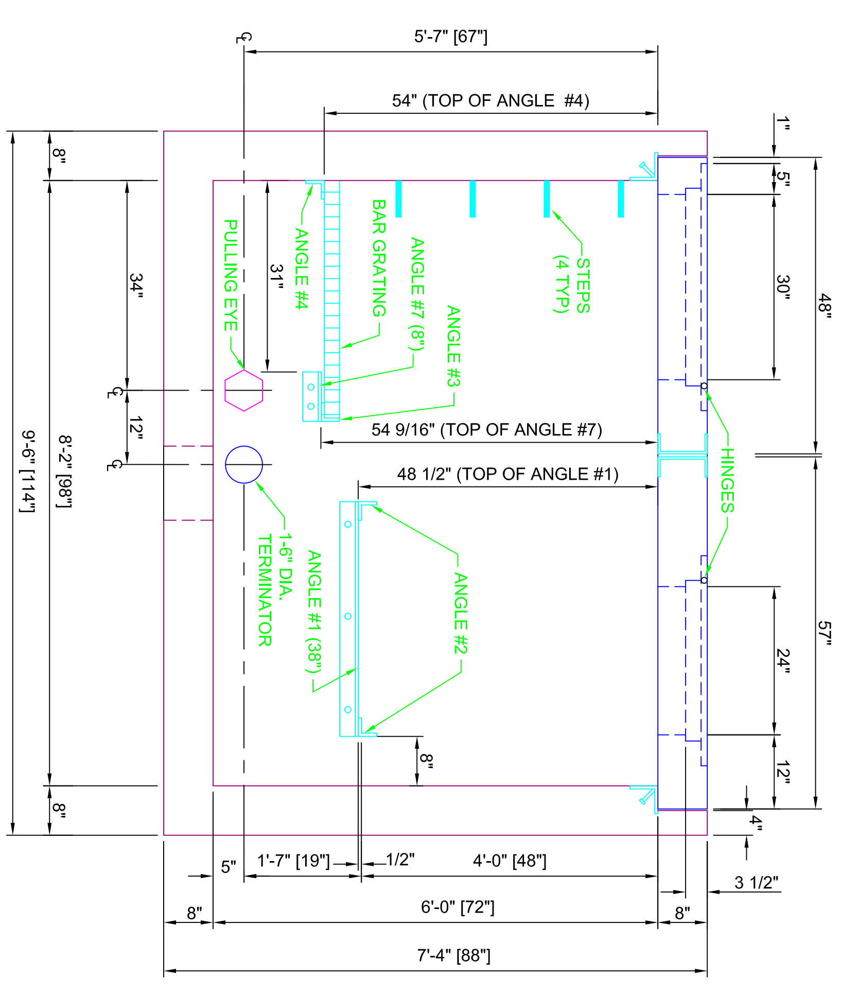
SECTION VIEW B-B (STANDING INSIDE BOX)
