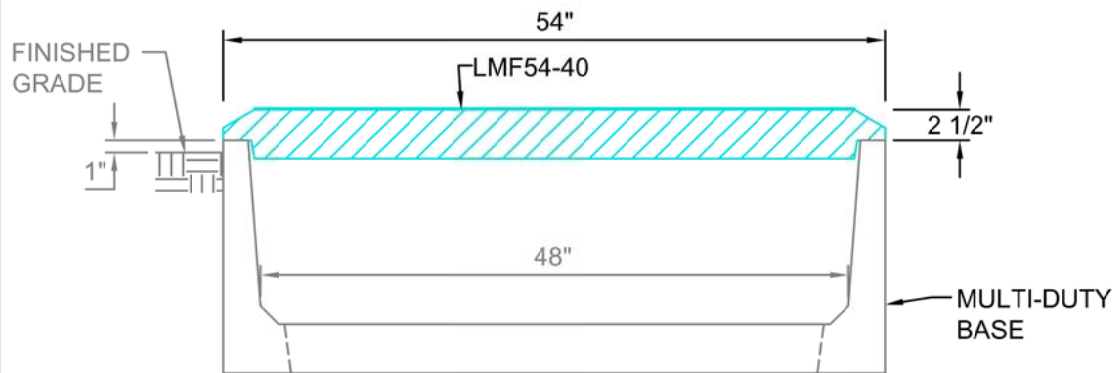
TIER 15 FIBRELITE LID ON MULTI-DUTY BASE
