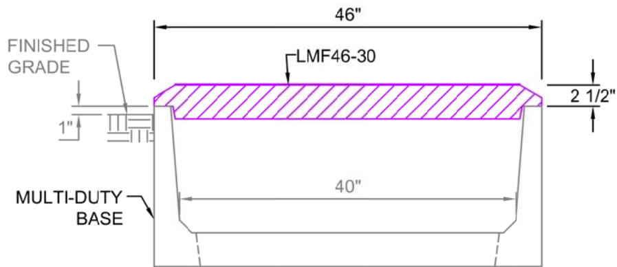
TIER 15 FIBRELITE LID ON MULTI-DUTY BASE
