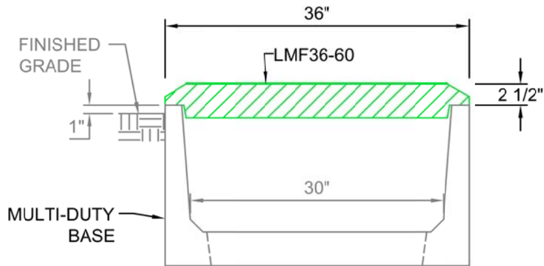
TIER 15 FIBRELITE LID ON MULTI-DUTY BASE
