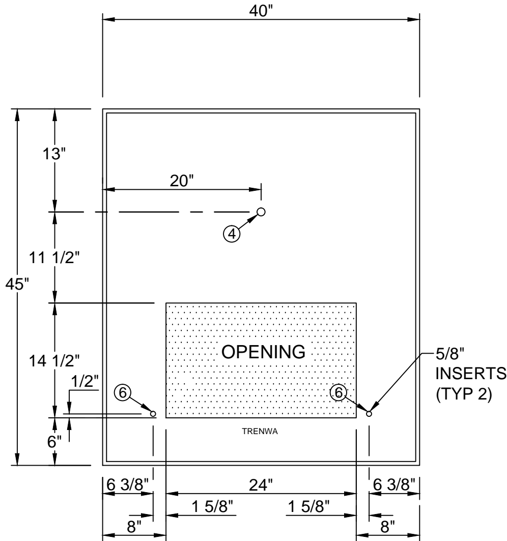
PLAN VIEW
