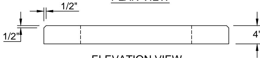
ELEVATION VIEW
