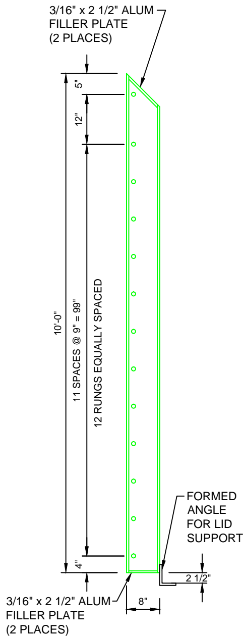
SIDE ELEVATION
