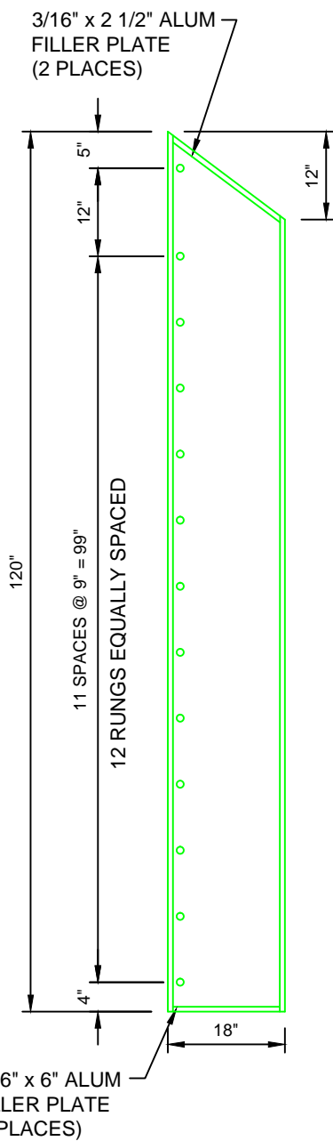
SIDE ELEVATION
