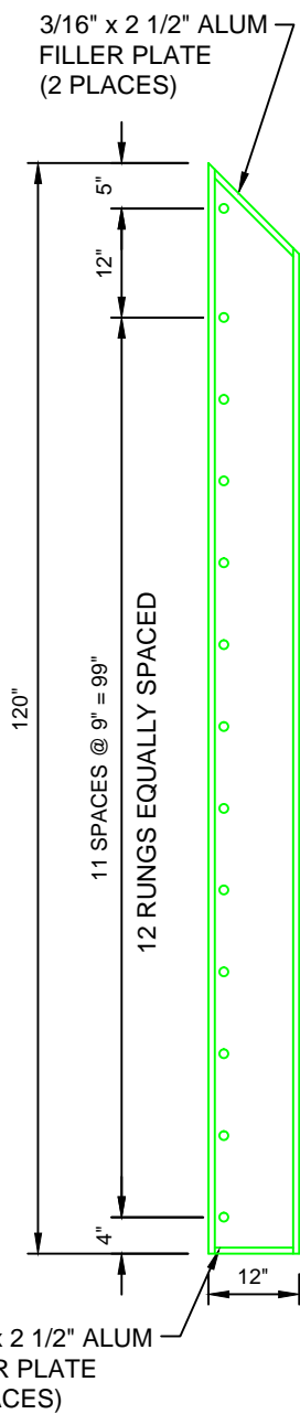
SIDE ELEVATION
