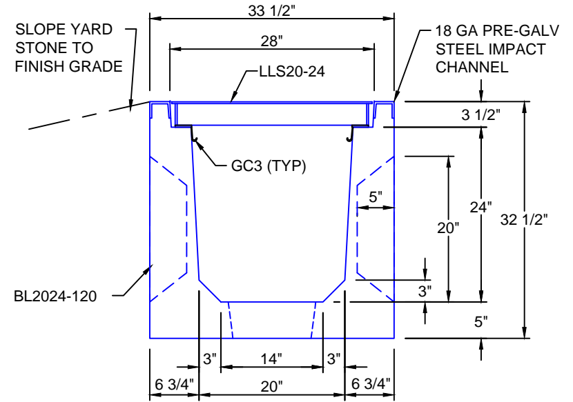
TYPICAL LIGHT TRAFFIC SECTION WITH STEEL LID 20"W x 24"D SCALE: 1" = 1'-0"
