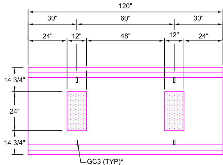
BHS4016-120 SCALE: 1/2" = 1'-0" WEIGHT: 4418
