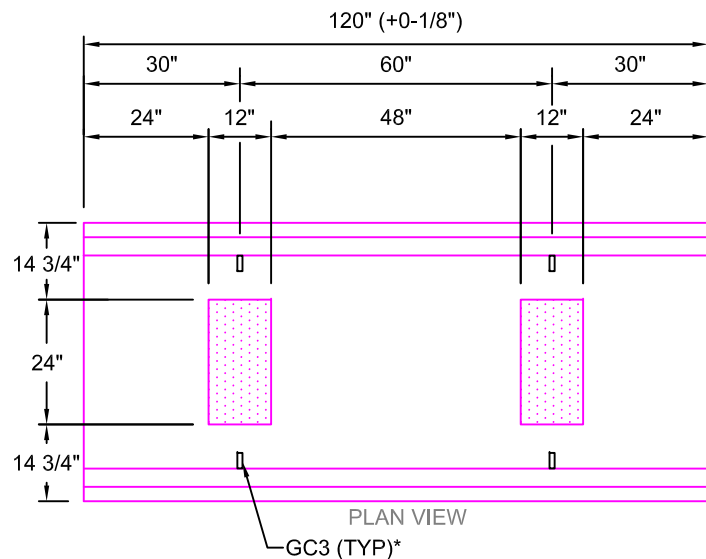
BHS4012-120 SCALE: 1/2" = 1'-0" WEIGHT: 3890 #
