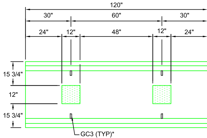
BHS3016-120 SCALE: 1/2" = 1'-0" WEIGHT: 4109
