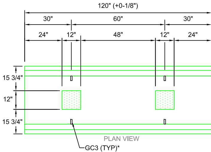
BHS3012-120 SCALE: 1/2" = 1'-0" WEIGHT: 3581 #
