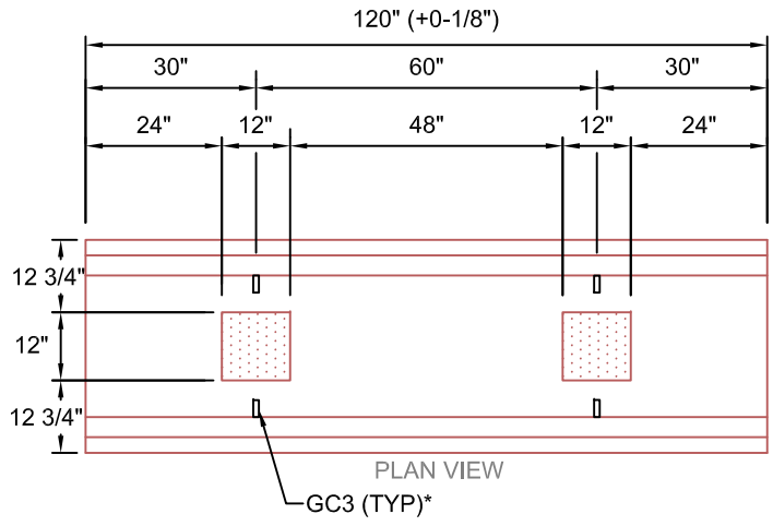
BHS2412-120 SCALE: 1/2" = 1'-0" WEIGHT: 3337 #
