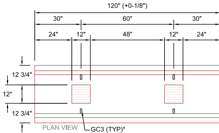
BHF2416-120 SCALE: 1/2" = 1'-0" WEIGHT: 3910#
