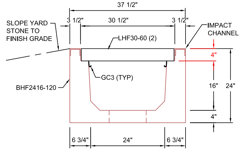
TYPICAL ROAD CROSSING SECTION WITH FIBRELITE LID 24"W x 16"D SCALE: 1"=1'-0"
