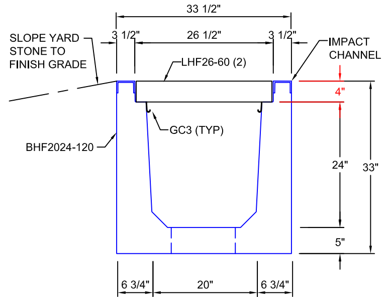
TYPICAL ROAD CROSSING SECTION WITH FIBRELITE LID 20"W x 24"D SCALE: 1"=1'-0"
