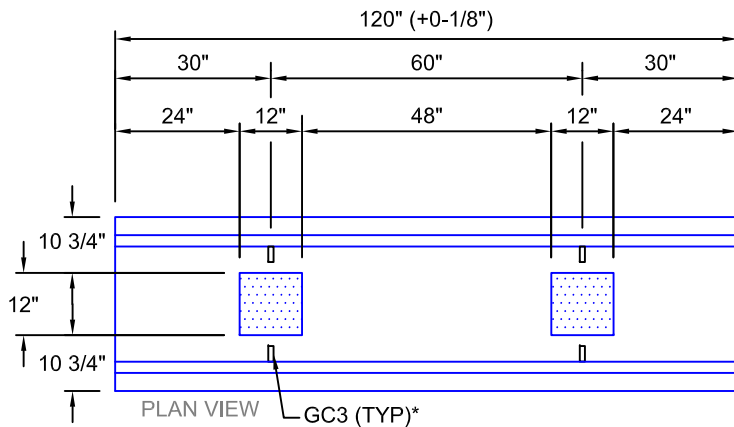
BHF2024-120 SCALE: 1/2" = 1'-0" WEIGHT: 5105#
