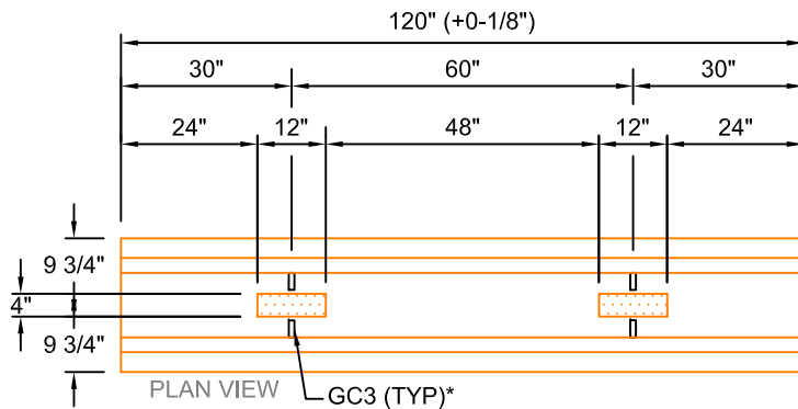
BHF1024-120 SCALE: 1/2" = 1'-0" WEIGHT: 4678#
