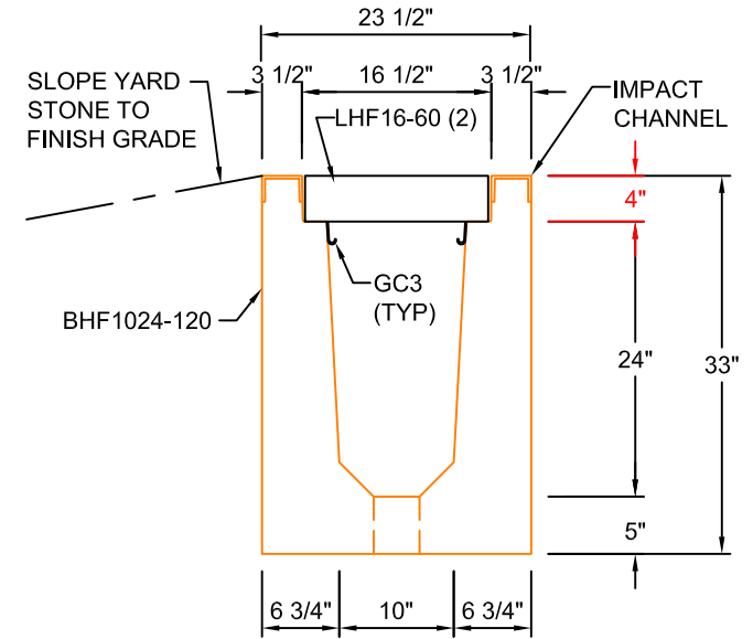
TYPICAL ROAD CROSSING SECTION WITH FIBRELITE LID 10"W x 24"D SCALE: 1"=1'-0"
