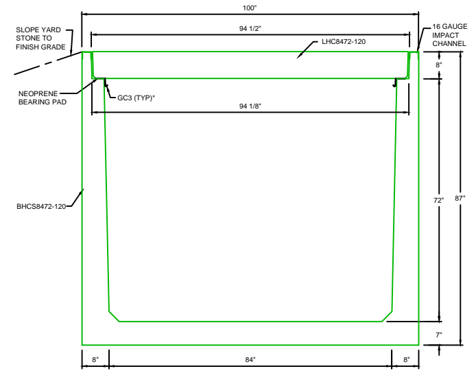
TYPICAL XL ROAD CROSSING SECTION 84"W x 72"D
