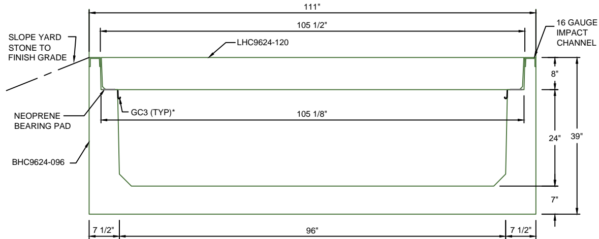
TYPICAL ROAD CROSSING SECTION 96"W x 24"D
