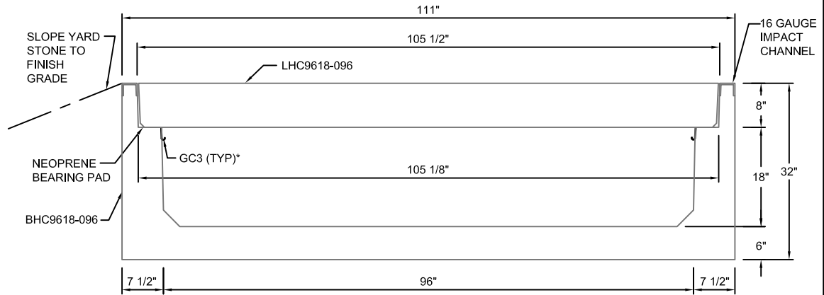
TYPICAL ROAD CROSSING SECTION 96"W x 18"D
