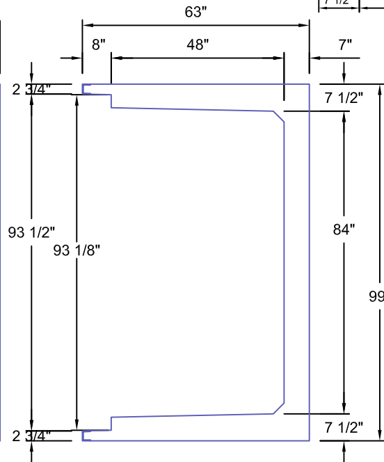
BHC8448-120 SCALE: 1/2"=1'-0"
