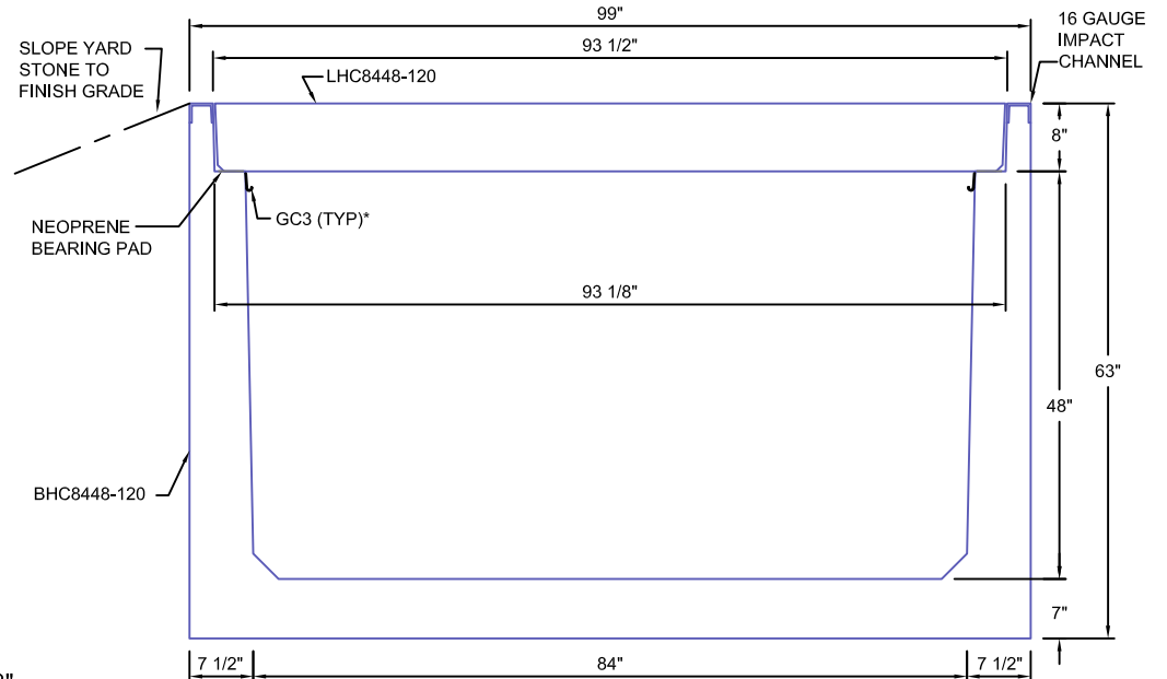
TYPICAL ROAD CROSSING SECTION 84"W x 48"D SCALE: 1/2"=1'-0"
