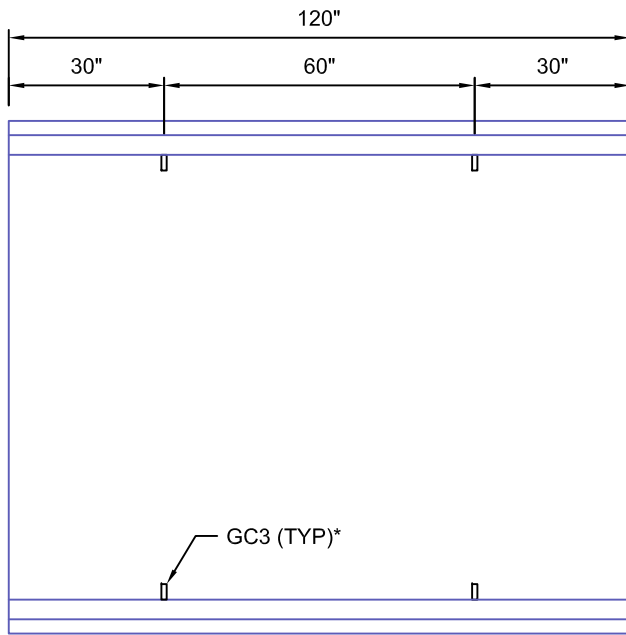
BHC8448-120 SCALE: 1/2"=1'-0"
