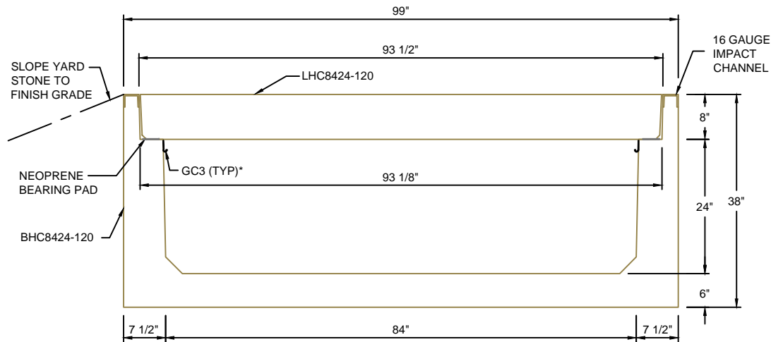
TYPICAL ROAD CROSSING SECTION 84"W x 24"D SCALE: 1"=1'-0"
