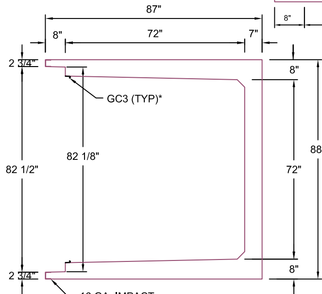
TYPICAL XL ROAD CROSSING SECTION 72"W x 72"D SCALE: 1"=1'-0"
