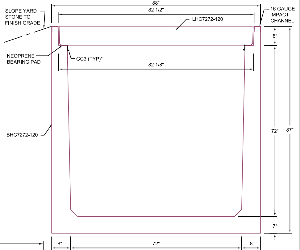
TYPICAL XL ROAD CROSSING SECTION 72"W x 72"D SCALE: 1"=1'-0"
