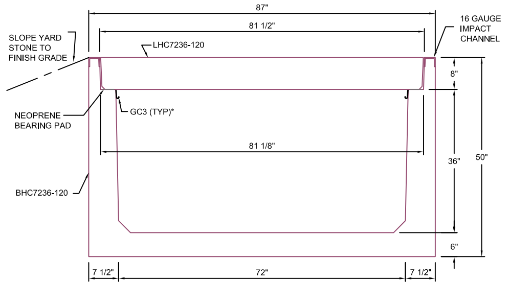
TYPICAL ROAD CROSSING SECTION 72"W x 36"D
