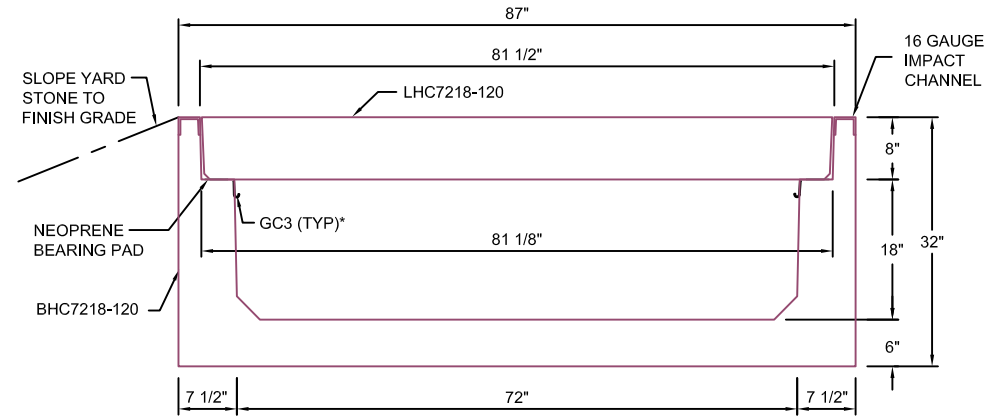
TYPICAL ROAD CROSSING SECTION 72"W x 18"D
