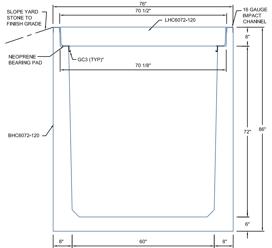
TYPICAL XL ROAD CROSSING SECTION 60"W x 72"D SCALE: 1"=1'-0"
