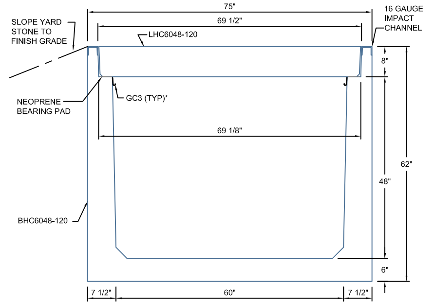
TYPICAL ROAD CROSSING SECTION 60"W x 48"D SCALE: 1"=1'-0"
