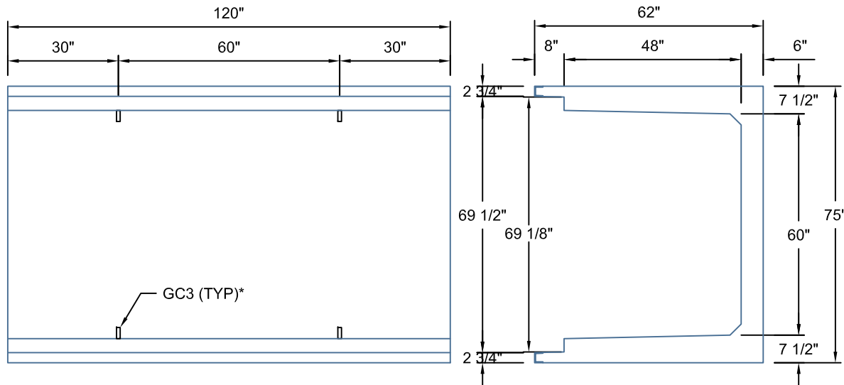
BHC6048-120 SCALE: 1/2"=1'-0"
