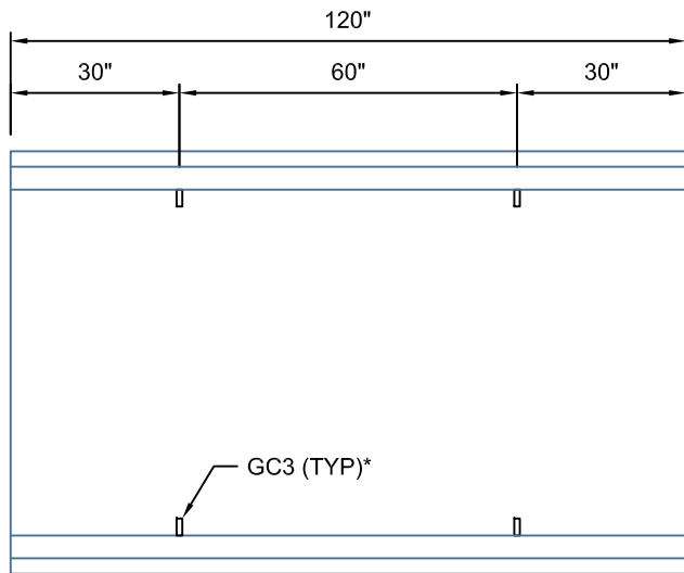
BHC6018-120 SCALE: 1/2"=1'-0"
