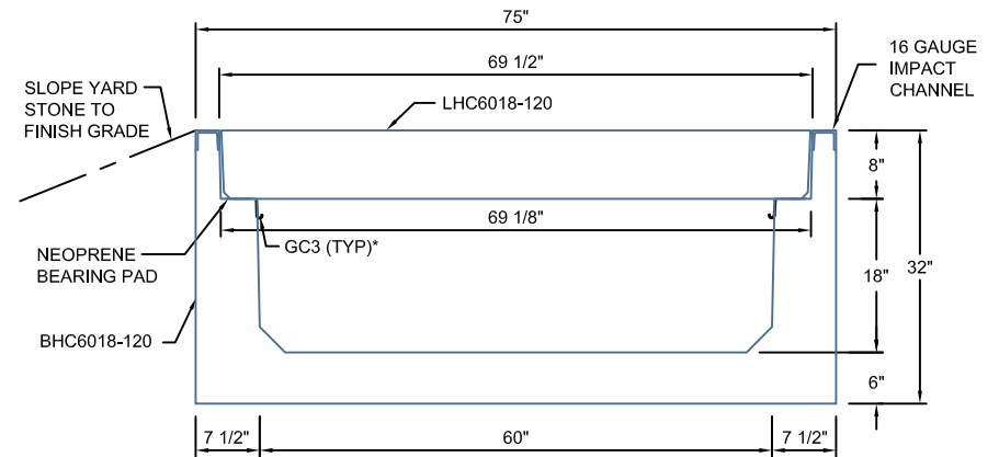
TYPICAL ROAD CROSSING SECTION 60"W x 18"D
