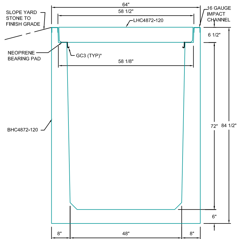
TYPICAL XL ROAD CROSSING SECTION 48"W x 72"D SCALE: 1"=1'-0"
