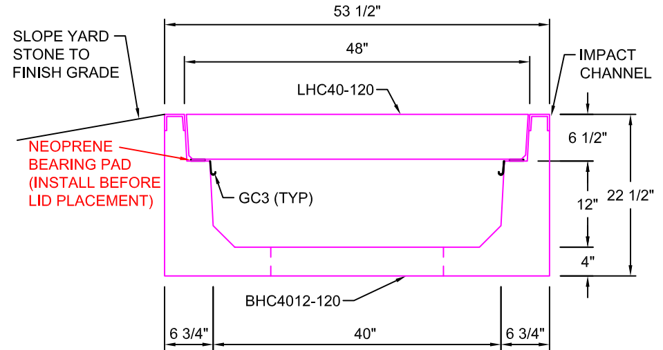
TYPICAL ROAD CROSSING SECTION 40"W x 12"D SCALE: 1"=1'-0"
