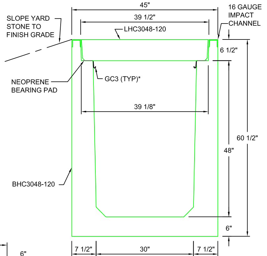
TYPICAL ROAD CROSSING SECTION 30"W x 48"D SCALE: 1"=1'-0"
