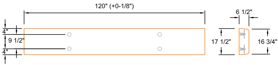
LHC10-120 SCALE: 1/2"=1'-0" WEIGHT: 1130 #
