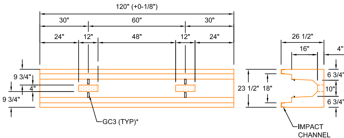
BHC1016-120 SCALE: 1/2" = 1'-0" WEIGHT: 3531#
