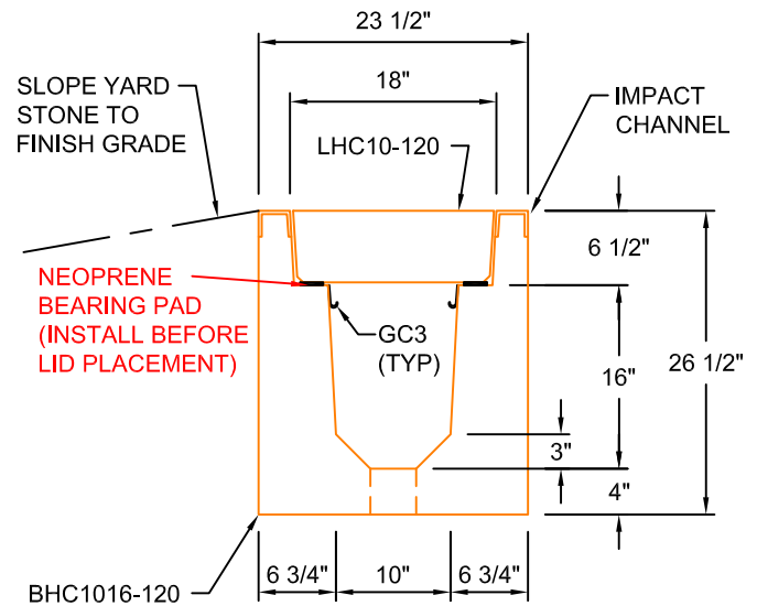
TYPICAL ROAD CROSSING SECTION 10"W x 16"D SCALE: 1"=1'-0"
