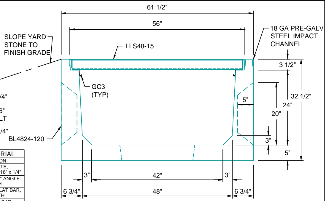
TYPICAL LIGHT TRAFFIC SECTION WITH STEEL LID 48"W x 24"D SCALE: 1" = 1'-0"
