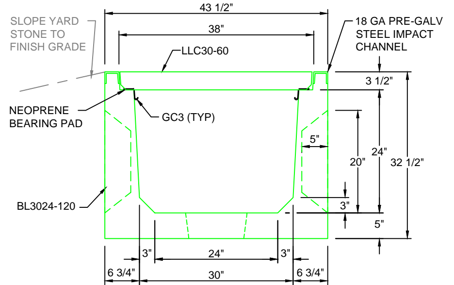
TYPICAL LIGHT TRAFFIC SECTION WITH CONCRETE LID 30"W x 24"D SCALE: 1" = 1'-0"
