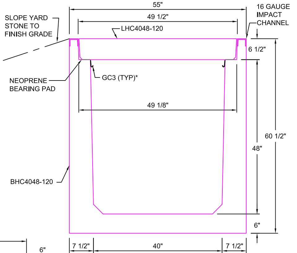
TYPICAL ROAD CROSSING SECTION 40"W x 48"D SCALE: 1"=1'-0"
