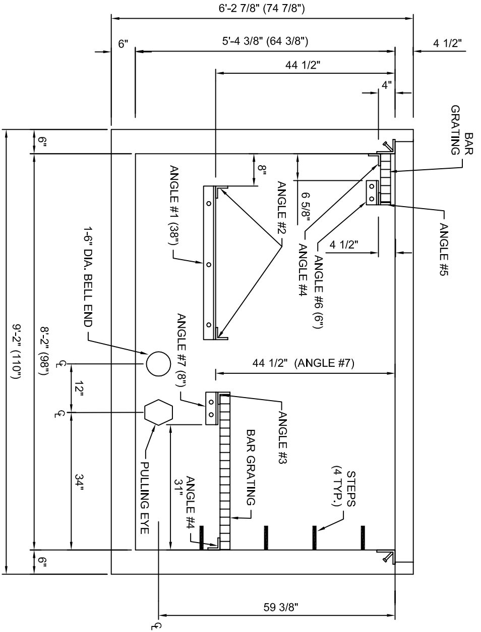
DETAIL SIDE "D" (STANDING INSIDE BOX)
