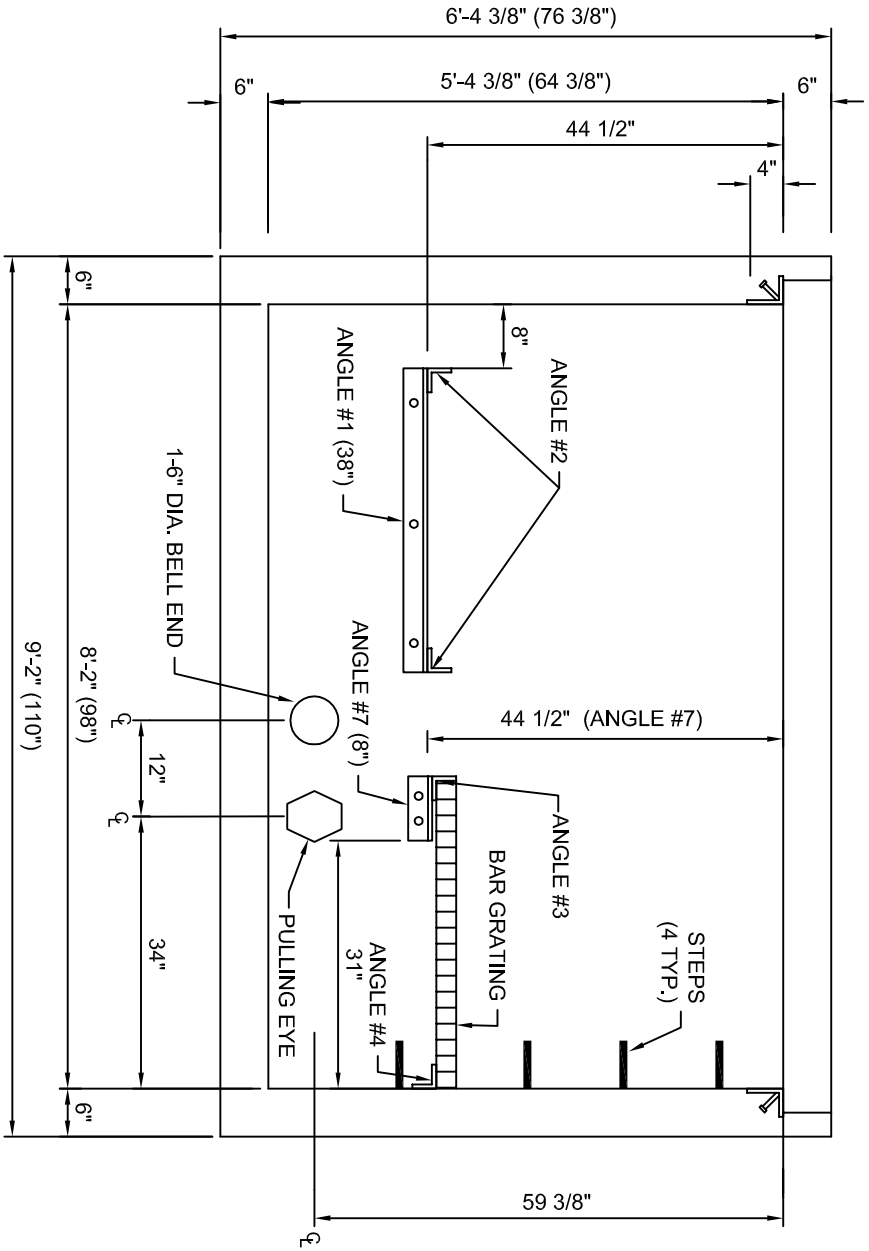
DETAIL SIDE "D" (STANDING INSIDE BOX)
