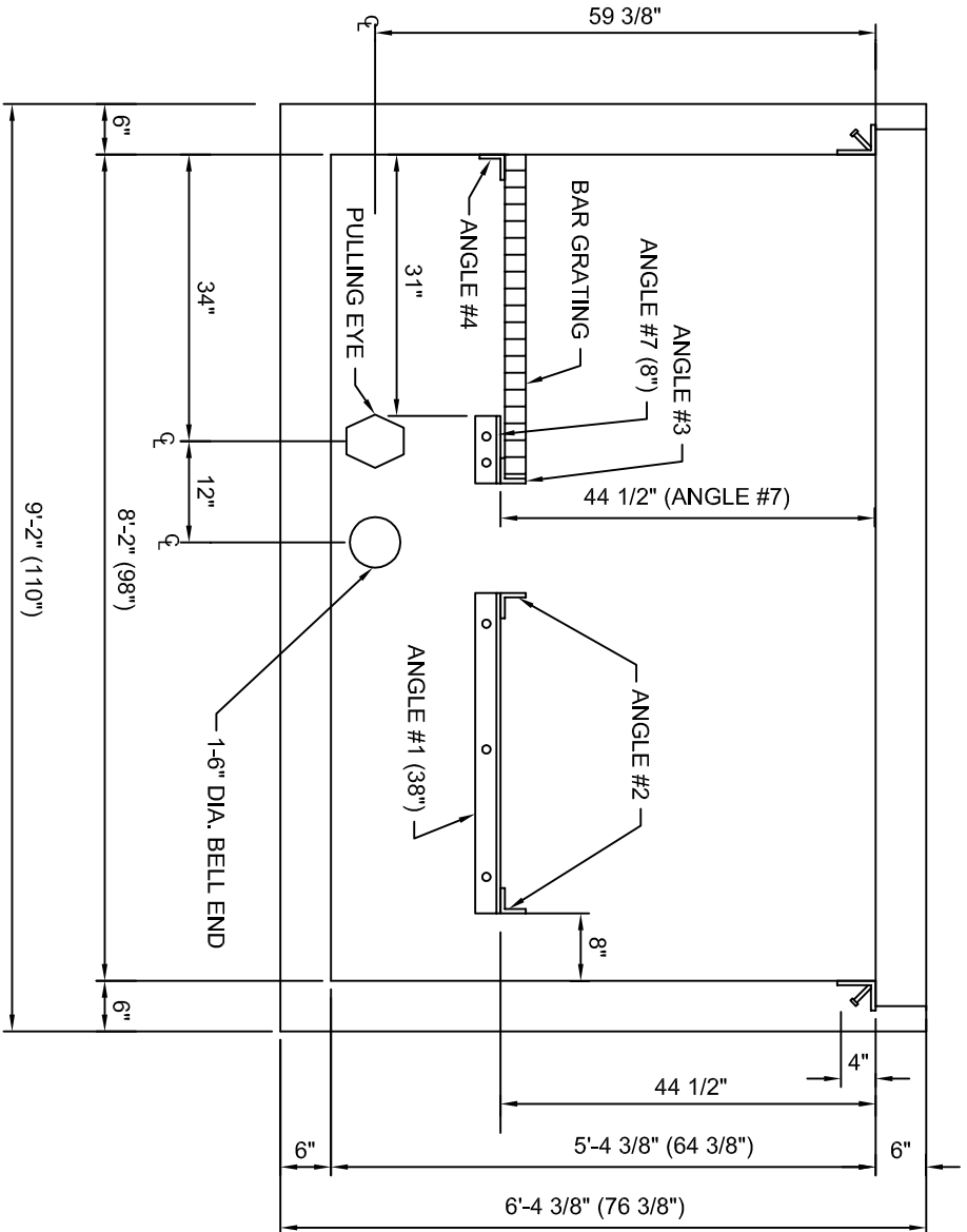
DETAIL SIDE "B" (STANDING INSIDE BOX)
