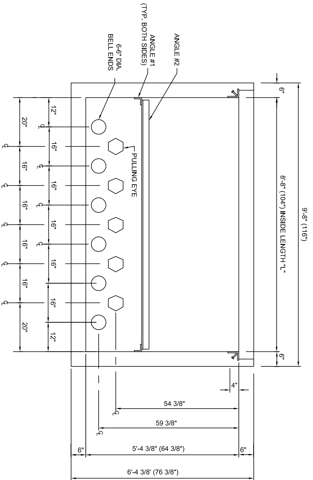
DETAIL SIDE "A" SWITCH GEAR END (STANDING INSIDE BOX)
