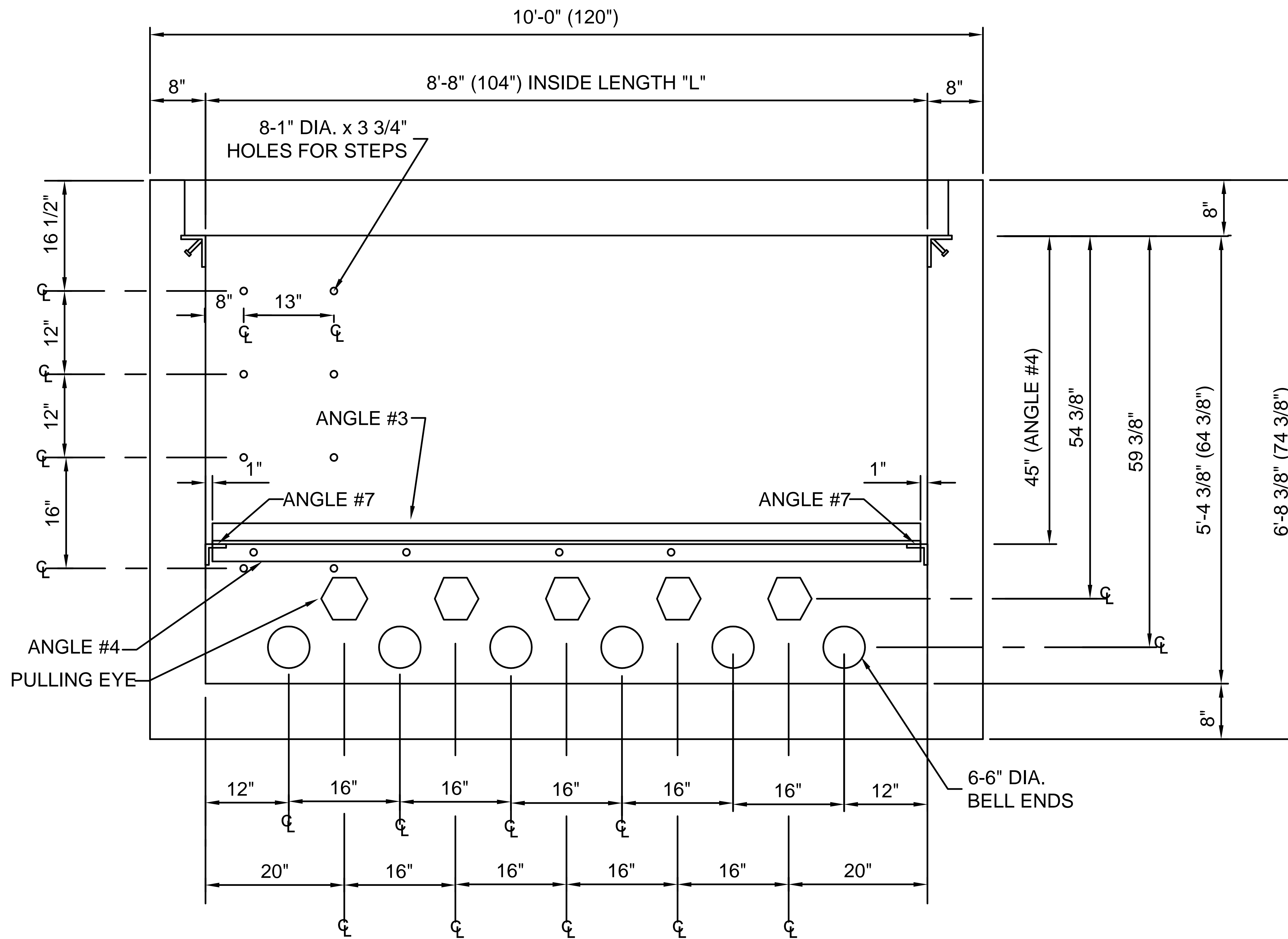
DETAIL SIDE "C"
